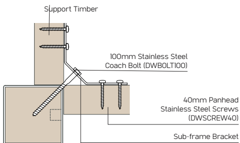
Fix bracket to post/post sleeve & sub-frame
