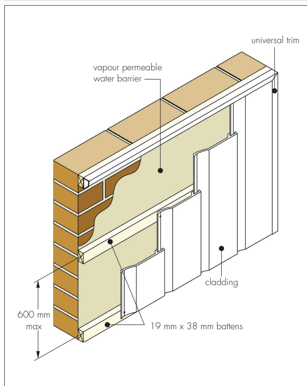
Figure 4 Vertical installation
