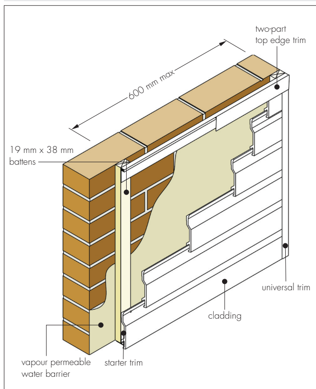
Figure 3 Horizontal installation
