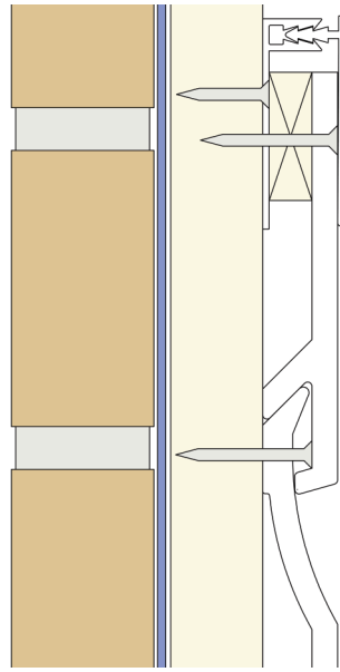
Two-part top edge trims — horizontal installation
